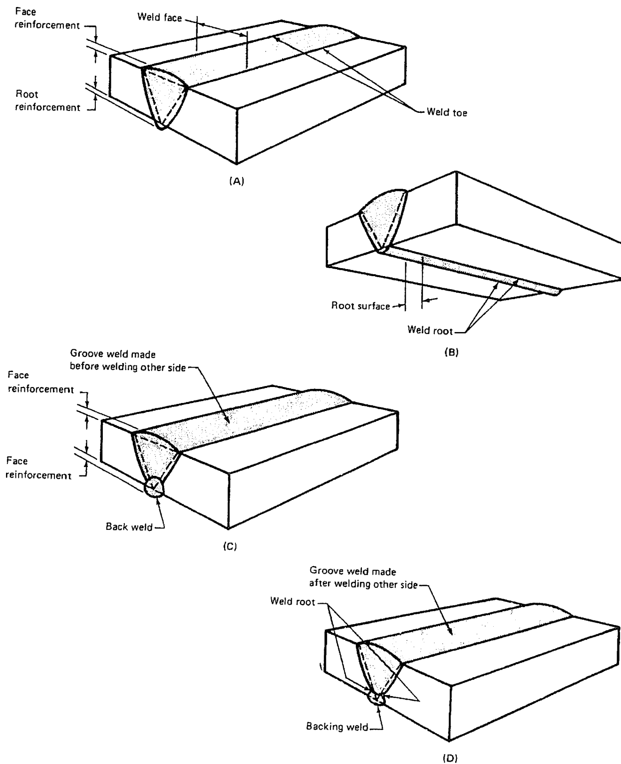
Fig. 17—Parts of a weld
