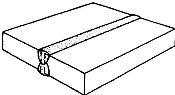
(A) Double-square-groove weld
