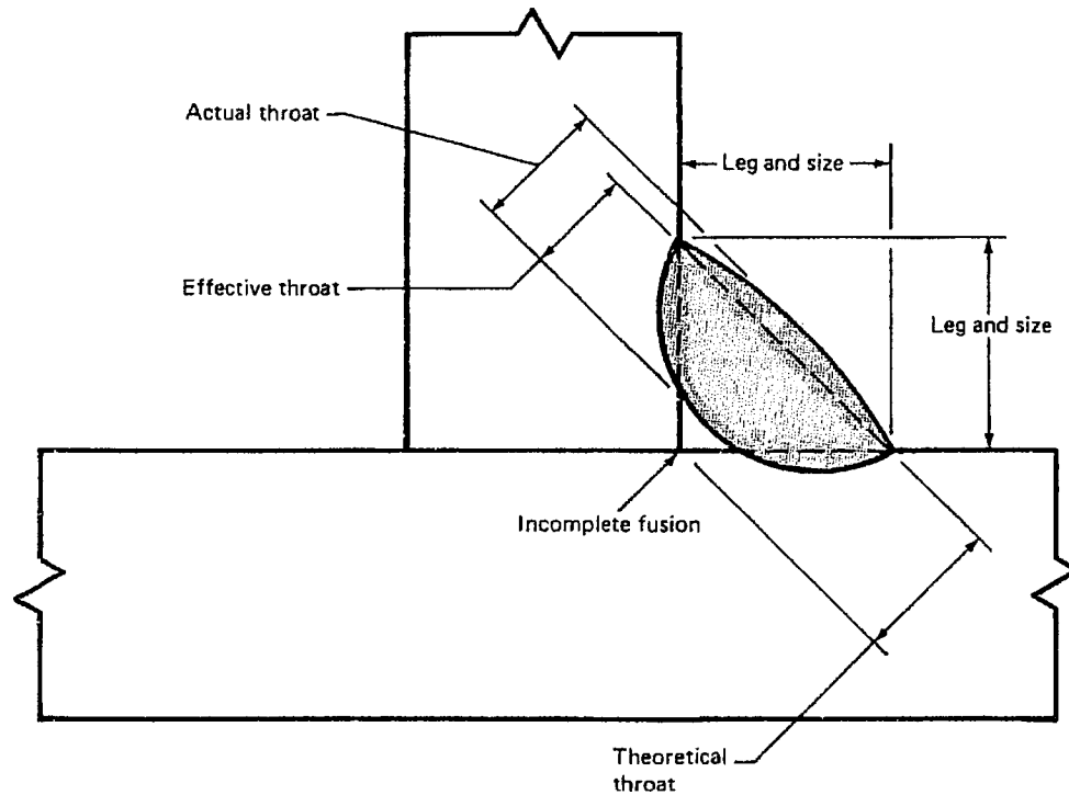
(C) Fillet weld with incomplete fusion
