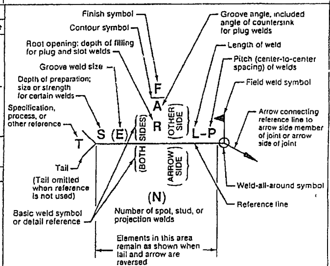
Location of Elements of a Welding Symbol
