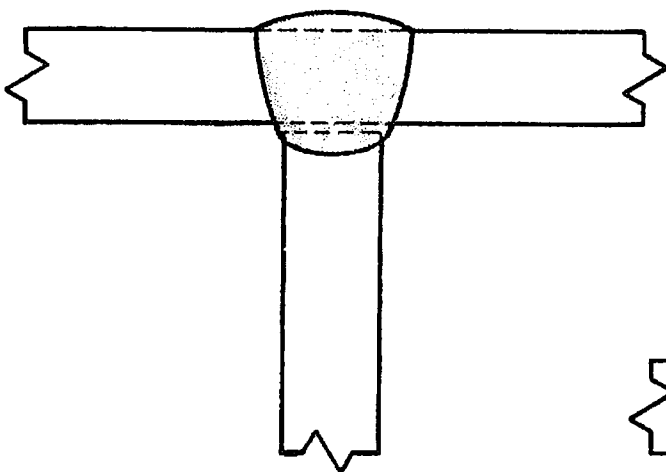
(L) Melt-through
