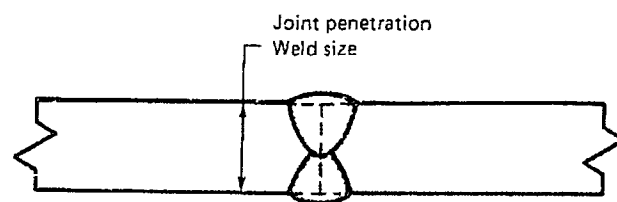
(F) Complete joint penetration
