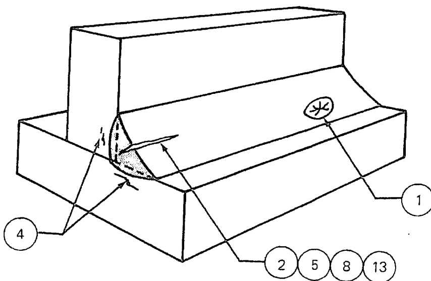
Fig. 25—Crack types
