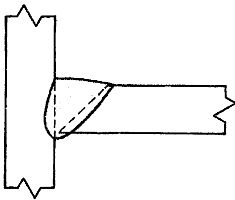
(J) Melt-through
