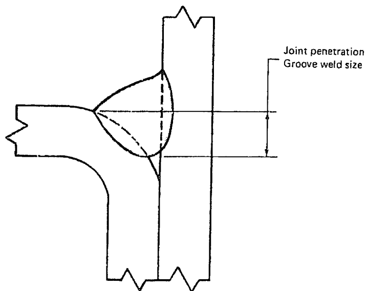
(H) Flare-bevel groove weld
