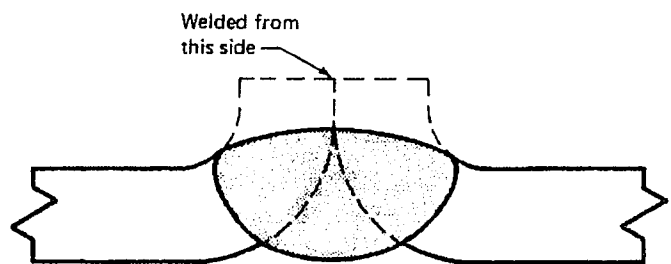
(M) Melt-through*
