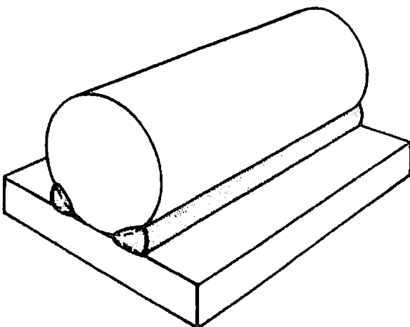
(F) Double-flare-bevel-groove weld
