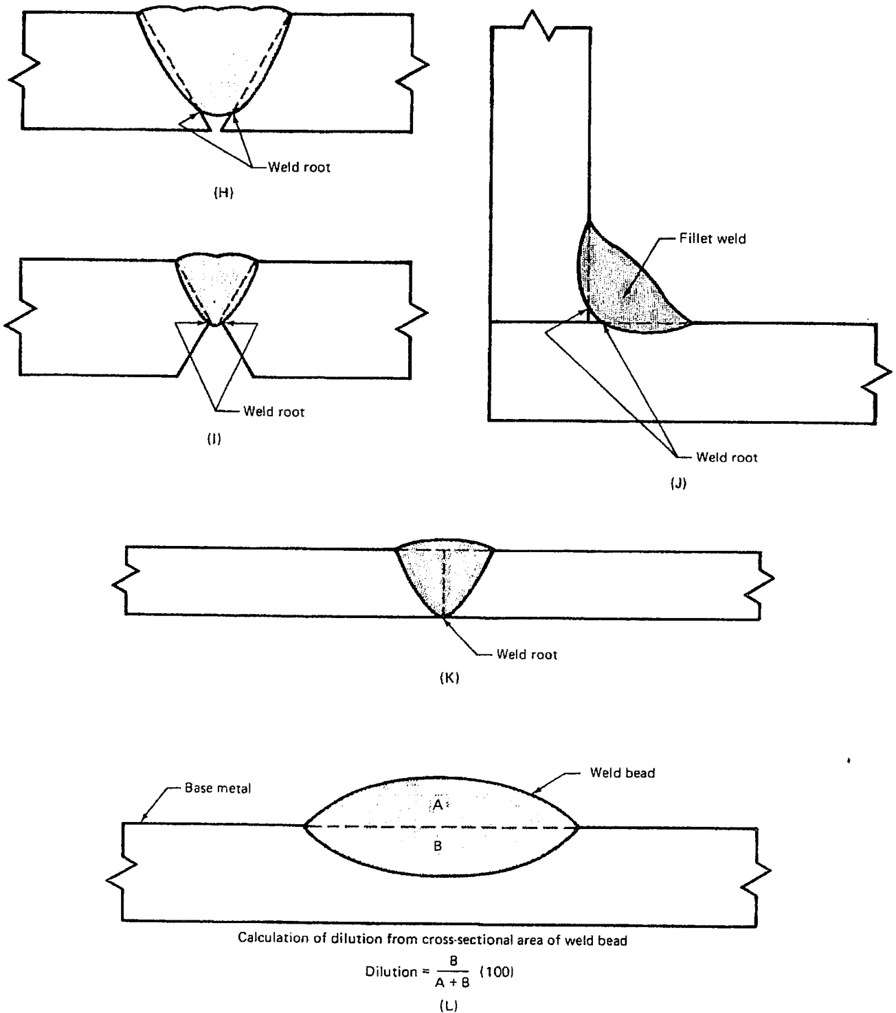
Fig. 17 (cont.)—Parts of a weld
