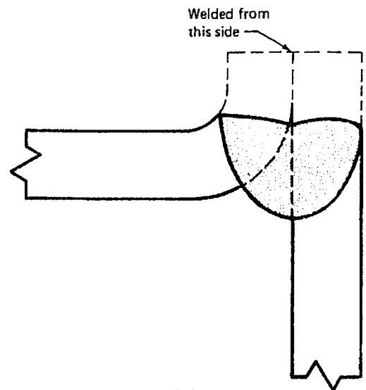
(K) Melt-through*
