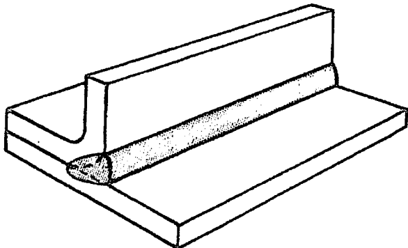
(G) Single-flare-bevel groove weld
