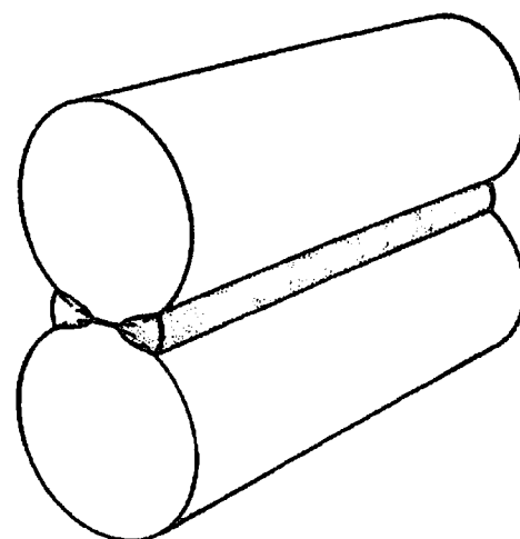
(G) Double-flare-V-groove weld
