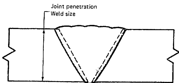
(G) Complete joint penetration
