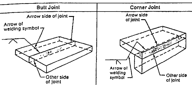
Basic Joints Identification of Arrow Side and Other Side of Joint
