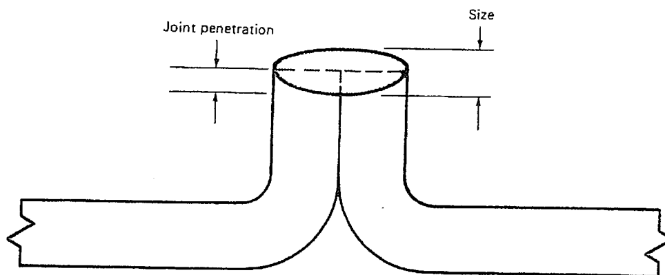
(G) Edge weld size or flange weld size
